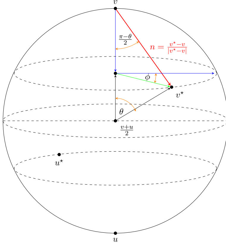
FIGURE 1. Parameterization of collisions
