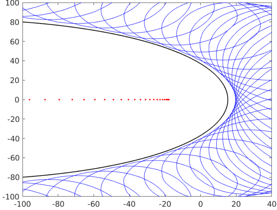
Figure 2: Pseudospectrum approximation for the advection-diffusion operator
