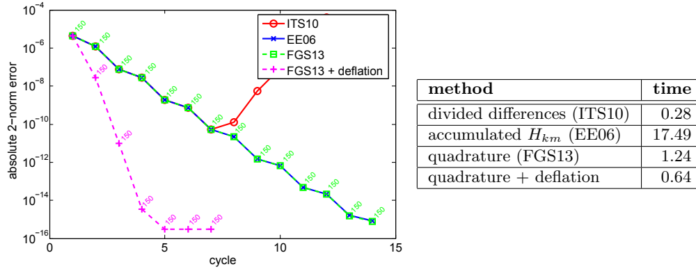
FIG. 5.4. Approximating (e^{-s\sqrt{A}} - I)A^{-1}\mathbf{b} : Convergence history (left) and running times (right) for the different restarting procedures. The restart length is m = 50 in all cases, and in the variant with deflation a number of d = 5 Ritz vectors was used.
